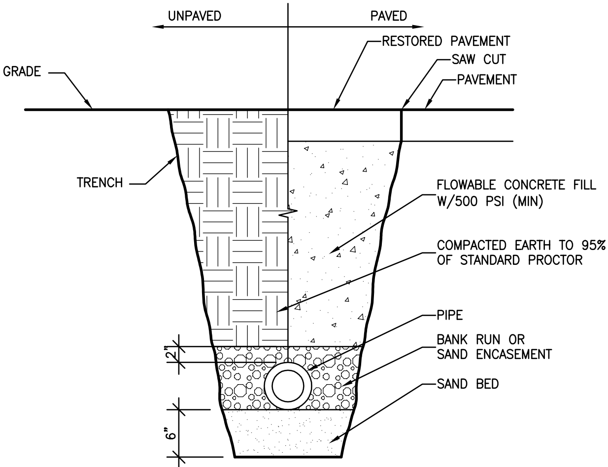
D5 TRENCH DETAIL A1.2 1"=1'-0"
