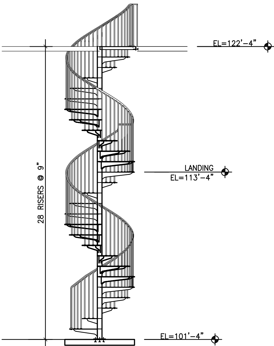
C1 SPIRAL STAIR 'B' ELEVATION A8.2 1/4"=1'-0"
