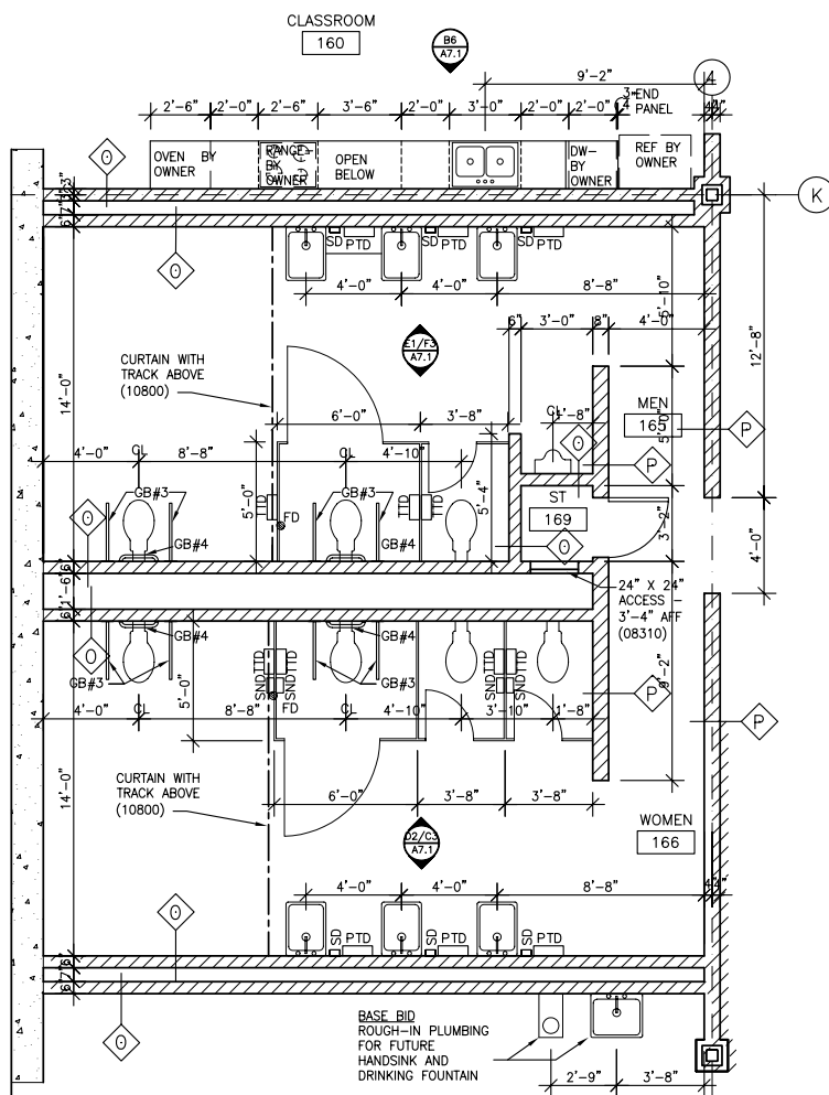
D2 TOILET ROOMS 165 & 166 A5.1 1/4" = 1'-0"
