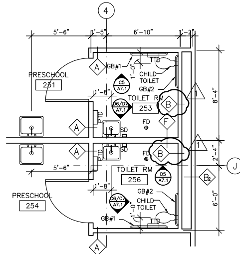
B2 TOILET ROOMS 253 & 256 A5.1 1/4" = 1'-0"
