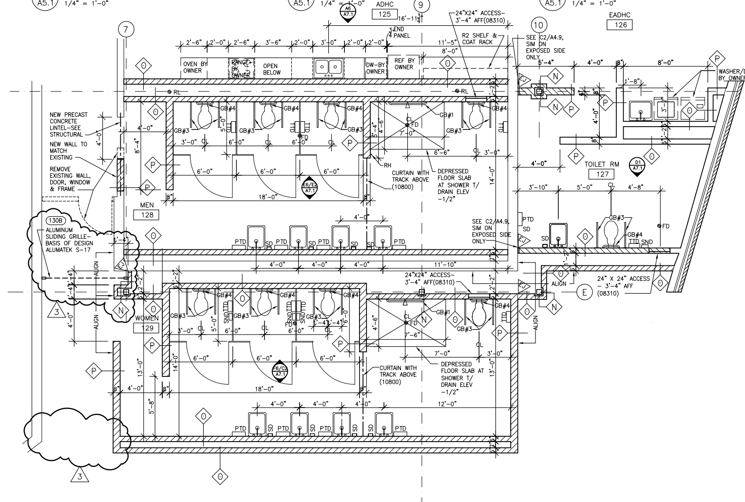
D3 TOILET ROOMS 127, 128 & 129 A5.1 1/4" = 1'-0"
