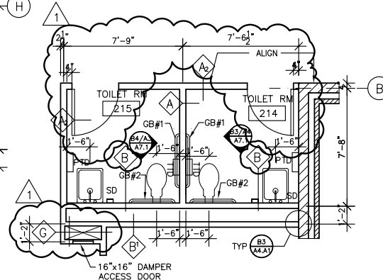
B4 TOILET ROOMS 215 & 214 A5.1 1/4" = 1'-0"
