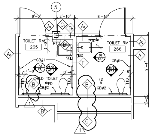
B3 TOILET ROOMS 265 & 266 A5.1 1/4" = 1'-0"
