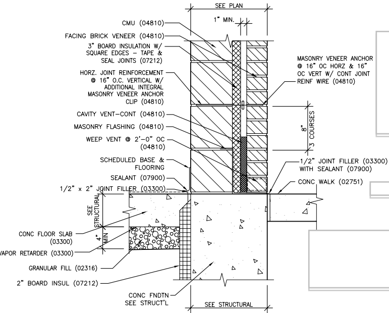
D3 TYPICAL CAVITY WALL A4.A1 1 1/2" = 1'-0"
